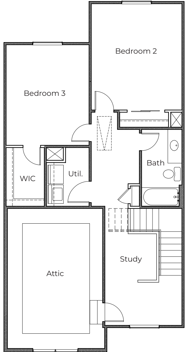
Second Floor
